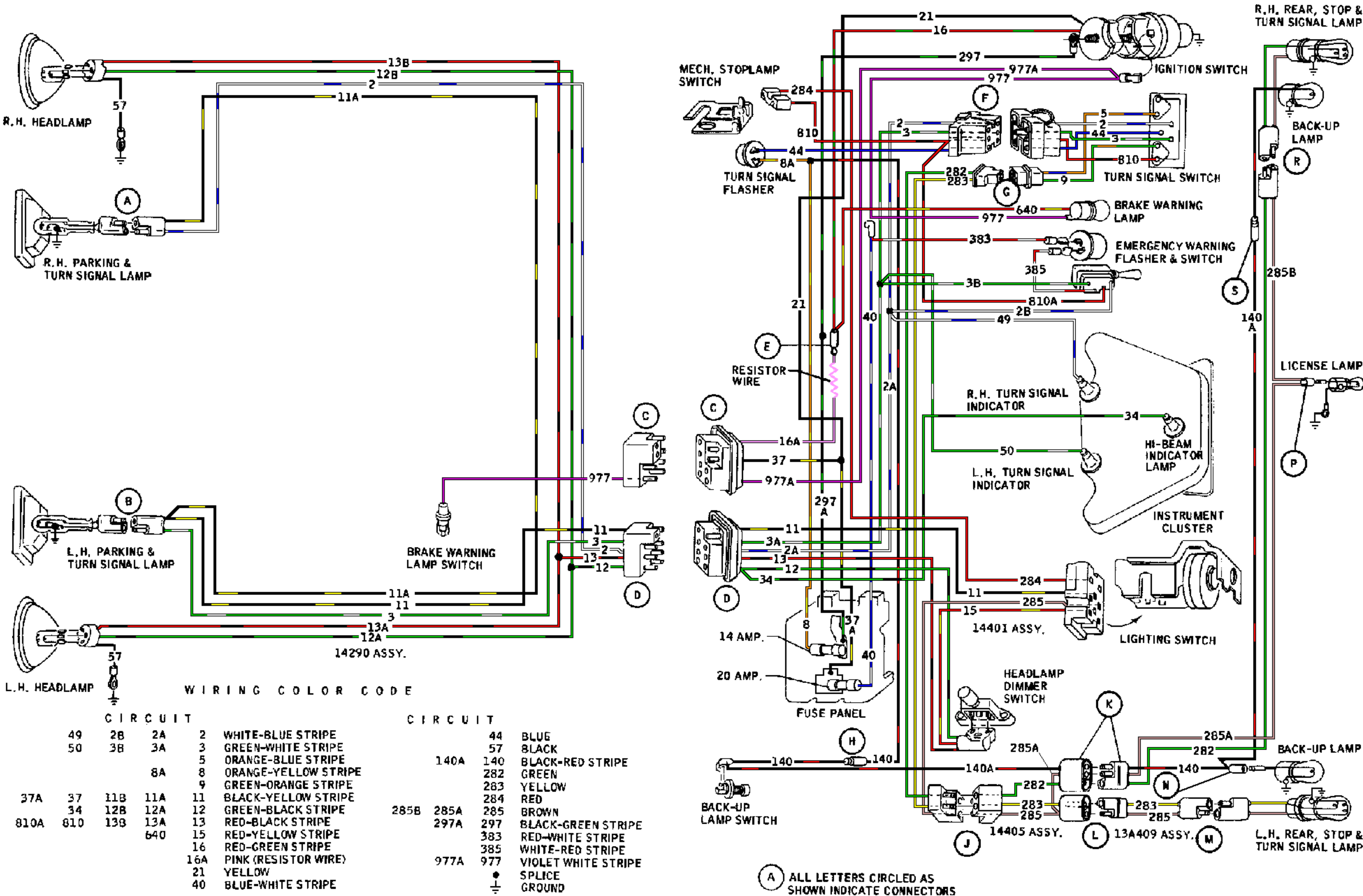
Wiring diagram for the exterior lights and turn signals—1967 Broncos *1966 should be similar
