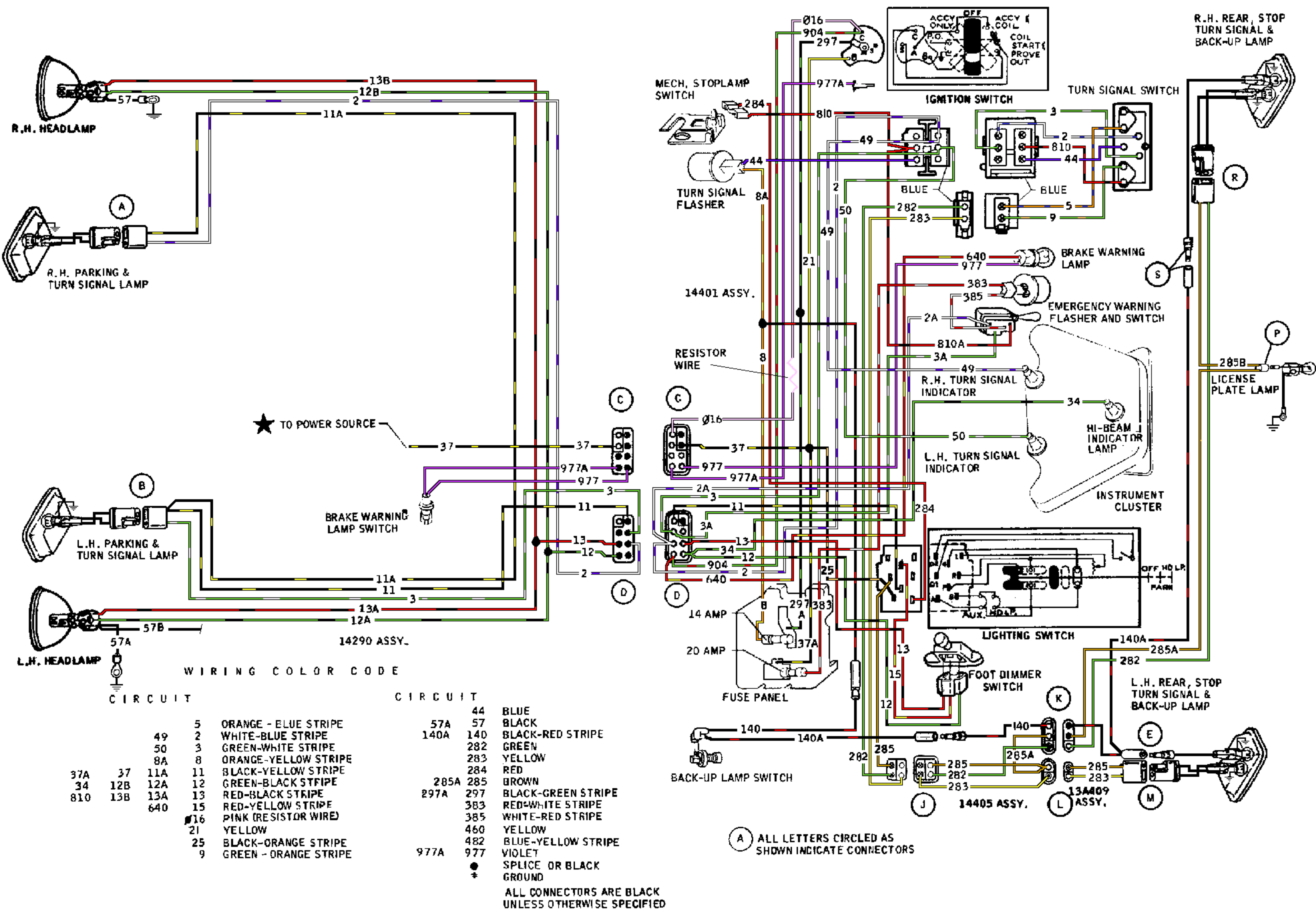
Wiring diagram for the exterior lights and turn signals—1969 Broncos *1968 is similar
