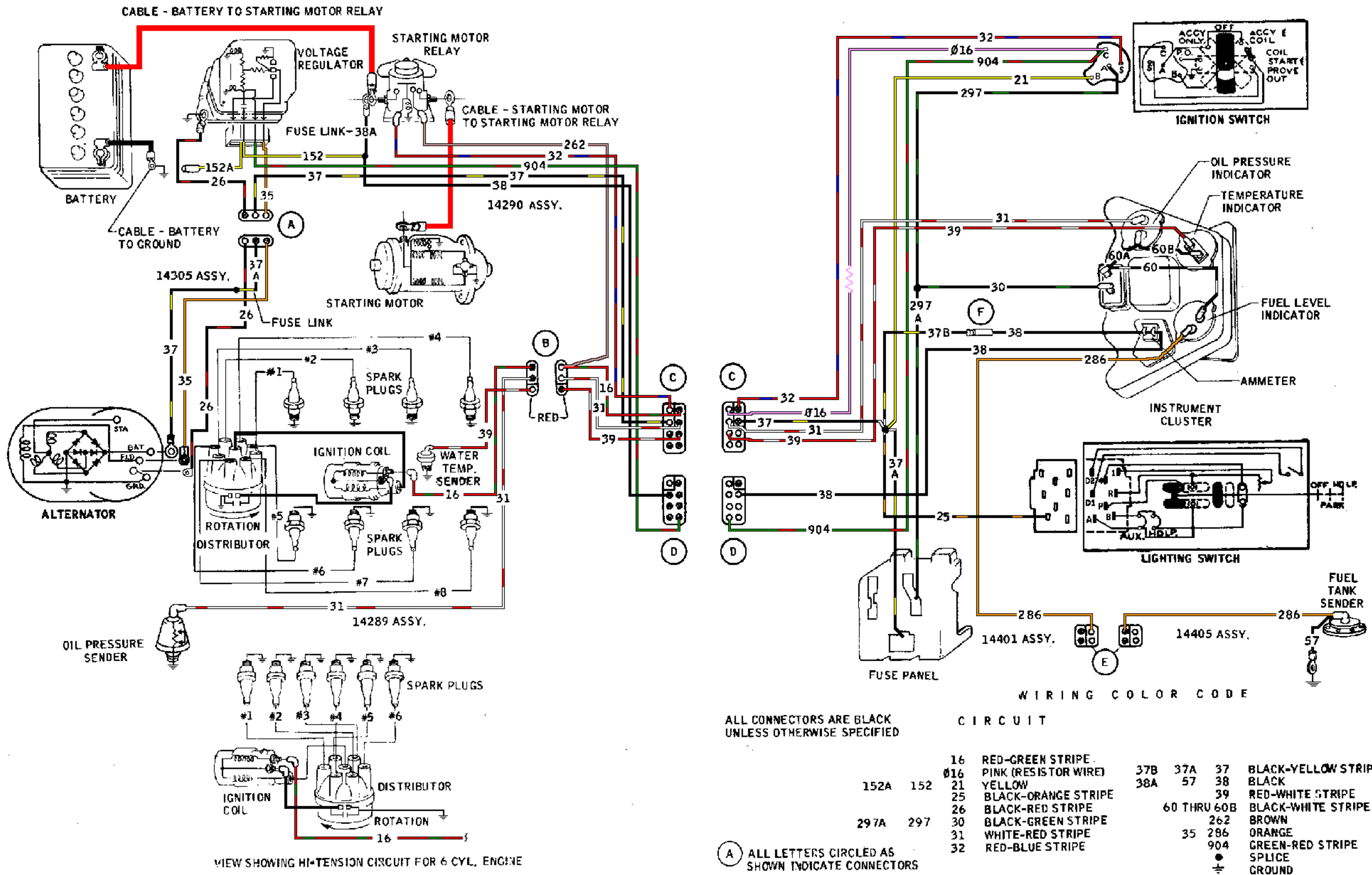
Wiring diagram for the ignition, starting, charging systems and gauges—1970 Broncos
