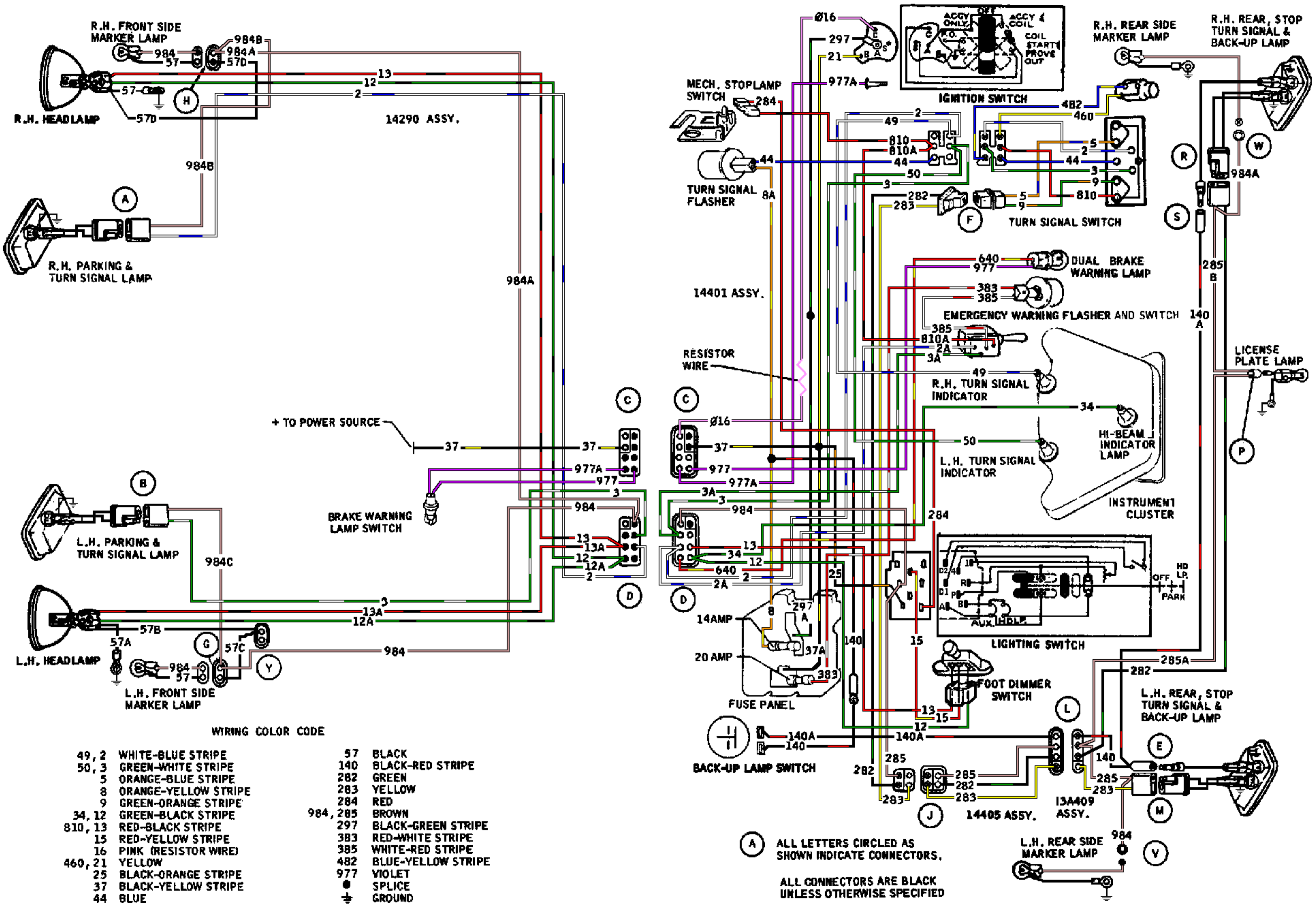
Wiring diagram for the exterior lights and turn signals—1970 Broncos
